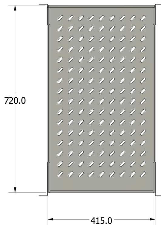
Bottom View
